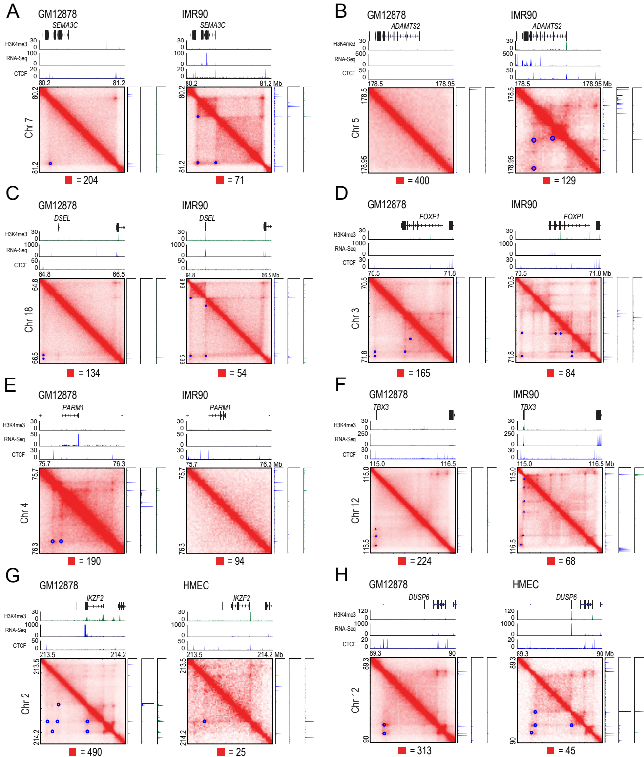
Data S1, VI. Cell-type Specific Loops and Gene Activation
