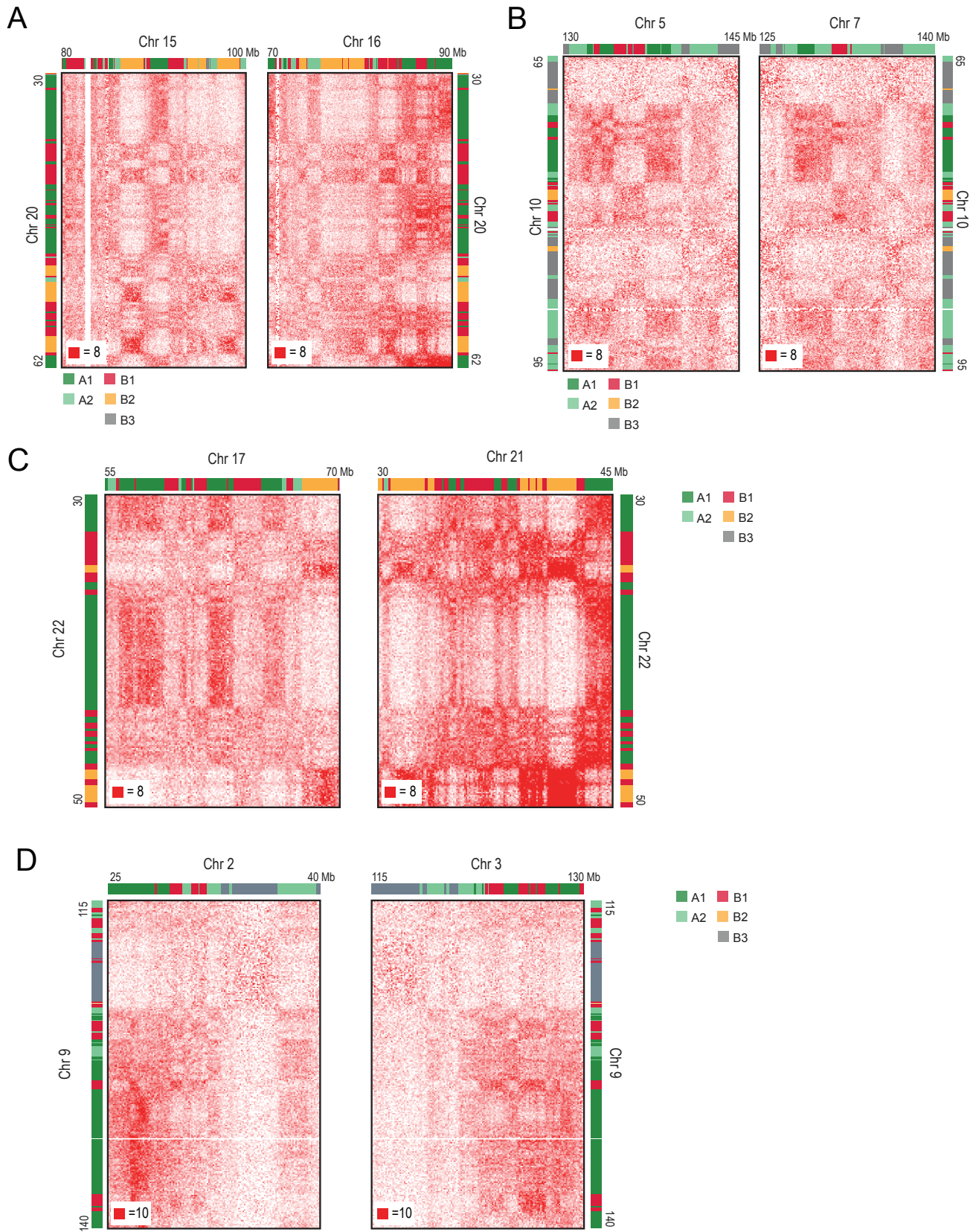
Data S1, IV. Subcompartment Interchromosomal Contact Patterns
