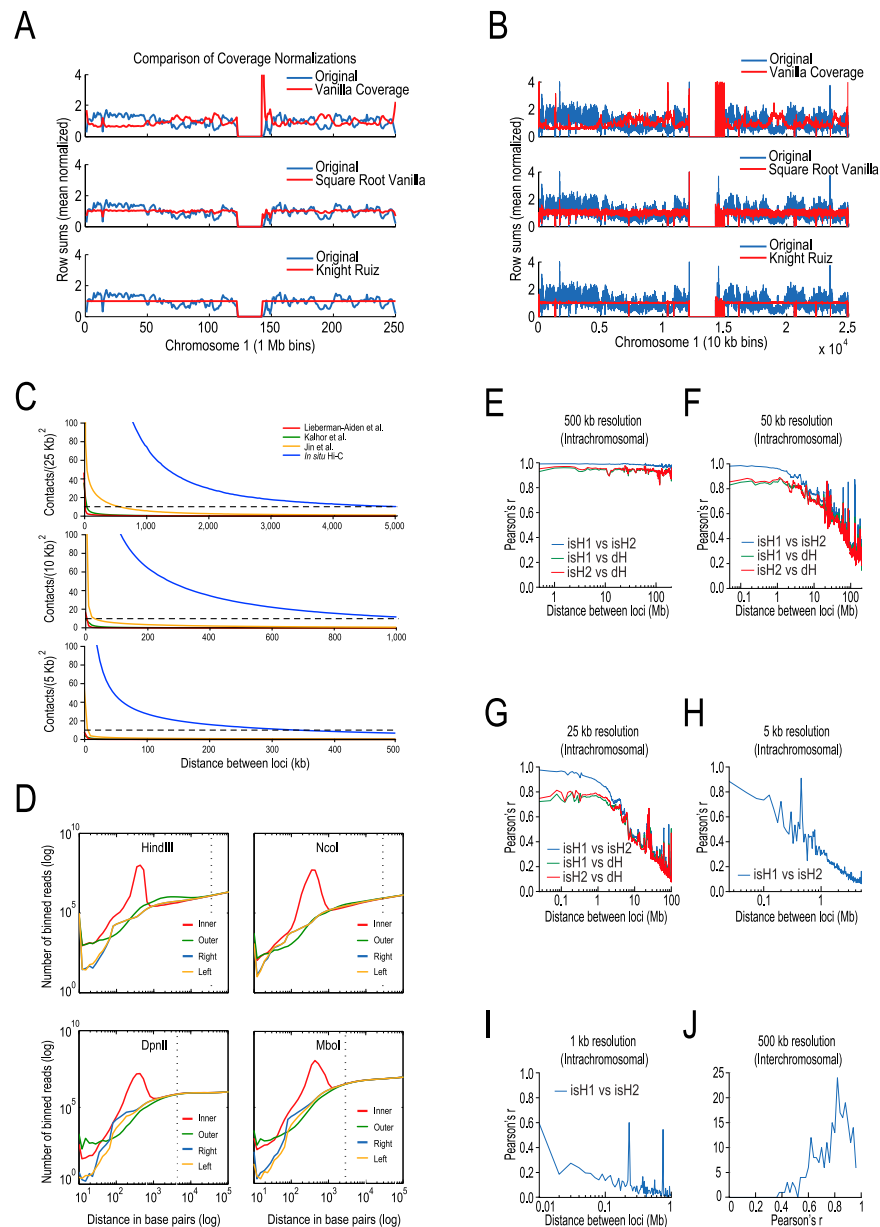
Figure S1. Robustness and Reproducibility of the In Situ Hi-C Protocol, Related to Figure 1
