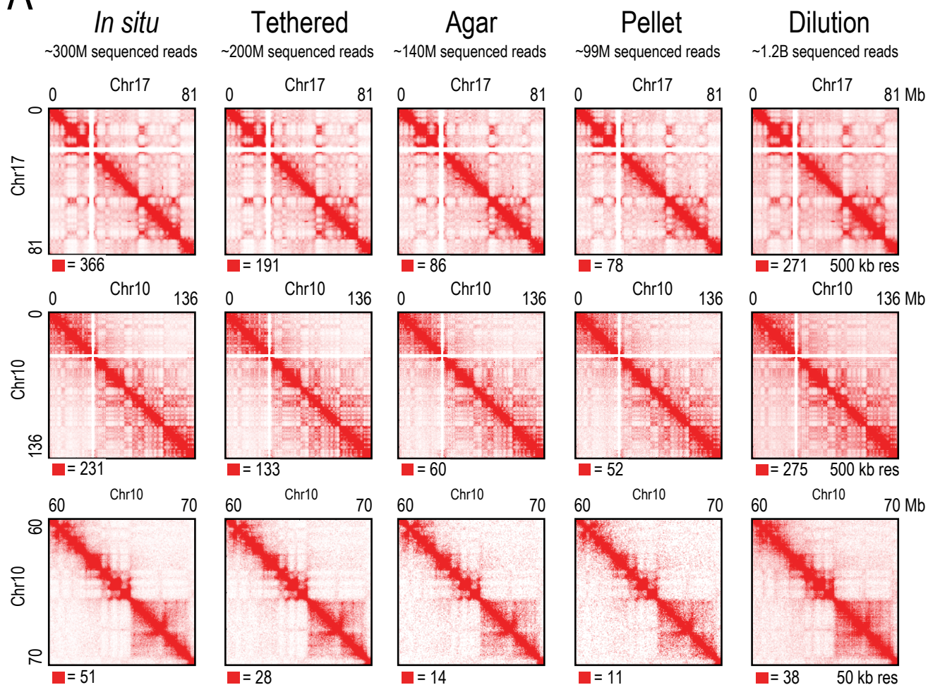
Data S1, I. Comparison of Hi-C Protocol Variants
