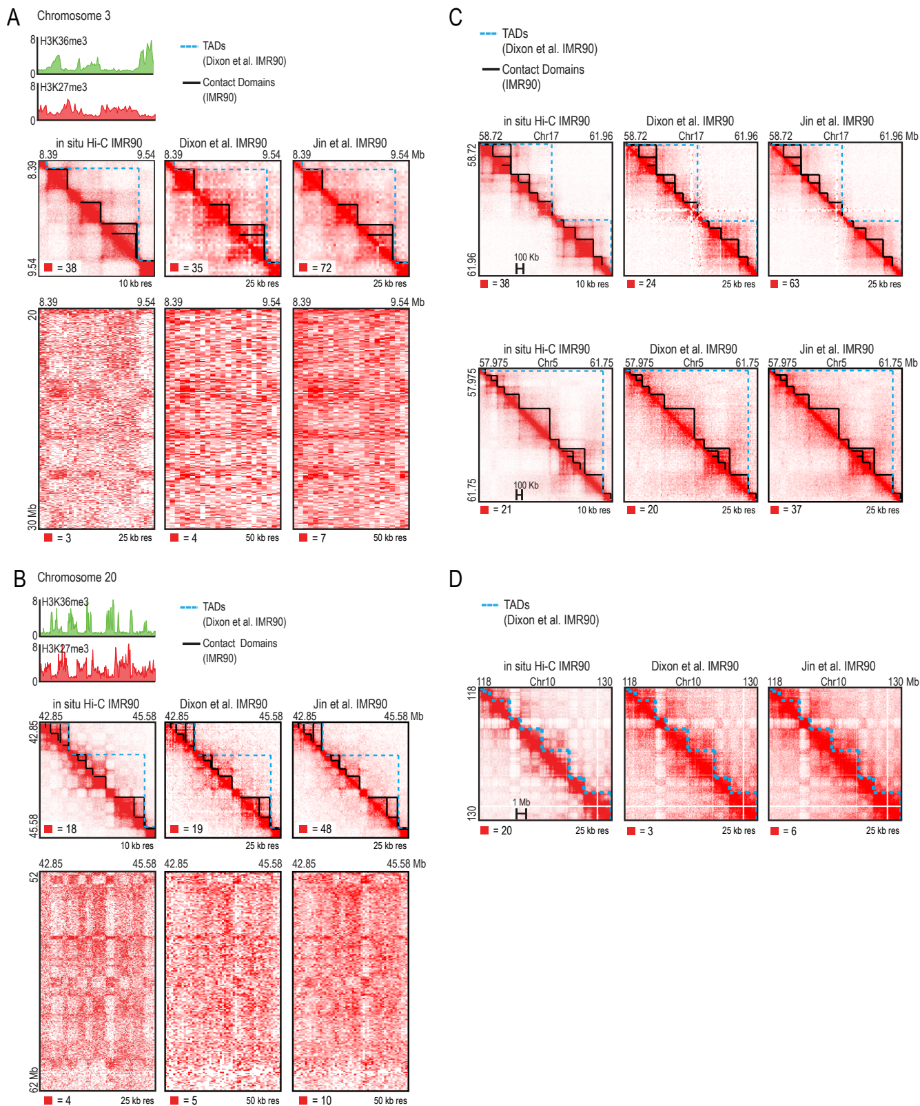
Data S1, III. Comparison of Contact Domains to TADs
