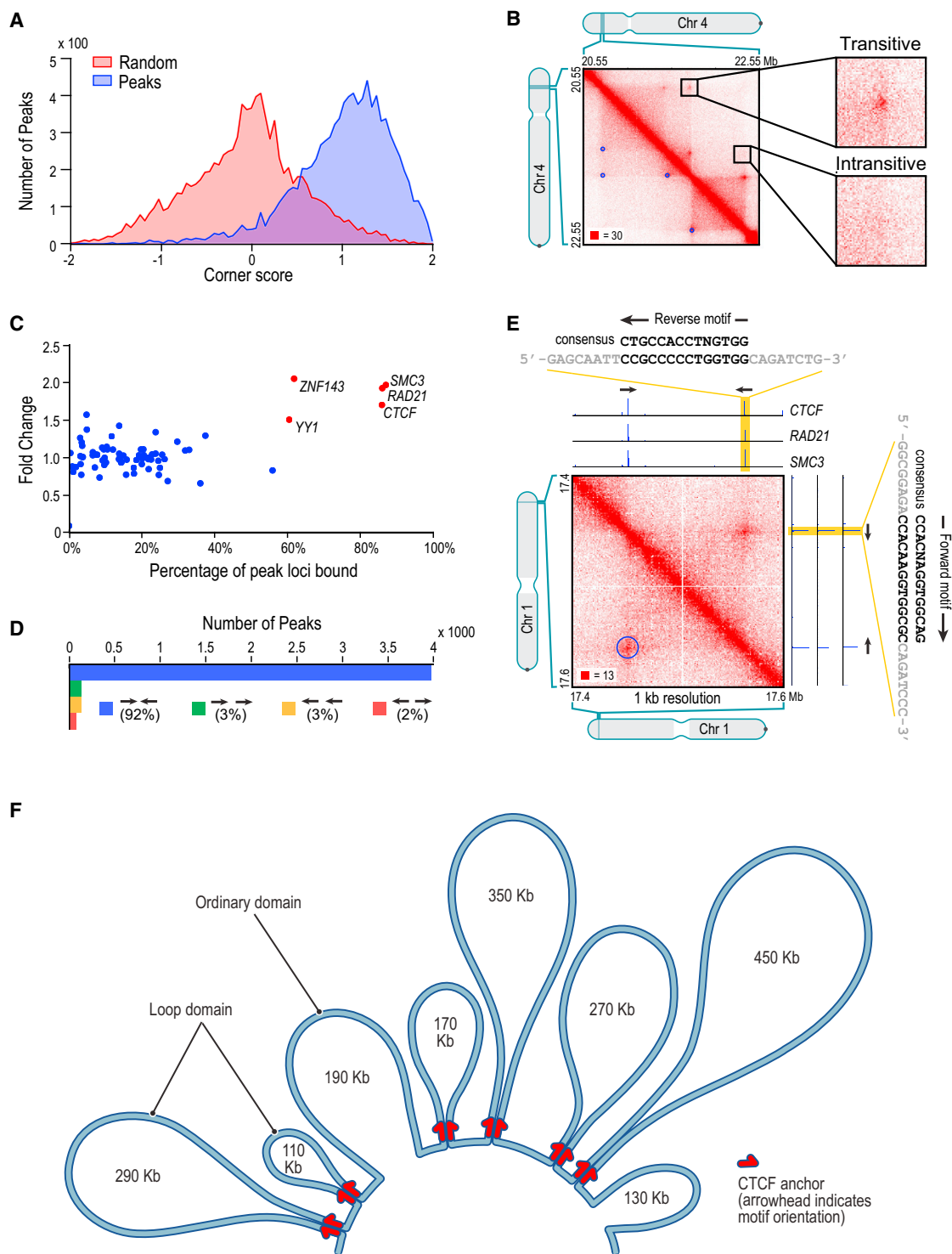
Figure 6. Many Loops Demarcate Contact Domains; The Vast Majority of Loops Are Anchored at a Pair of Convergent CTCF/RAD21/SMC3 Binding Sites
